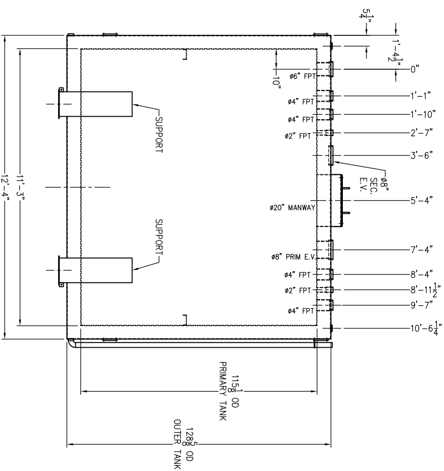
ELEVATION VIEW
