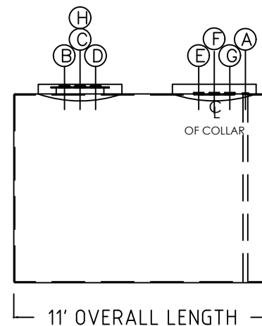
ELEVATION VIEW
