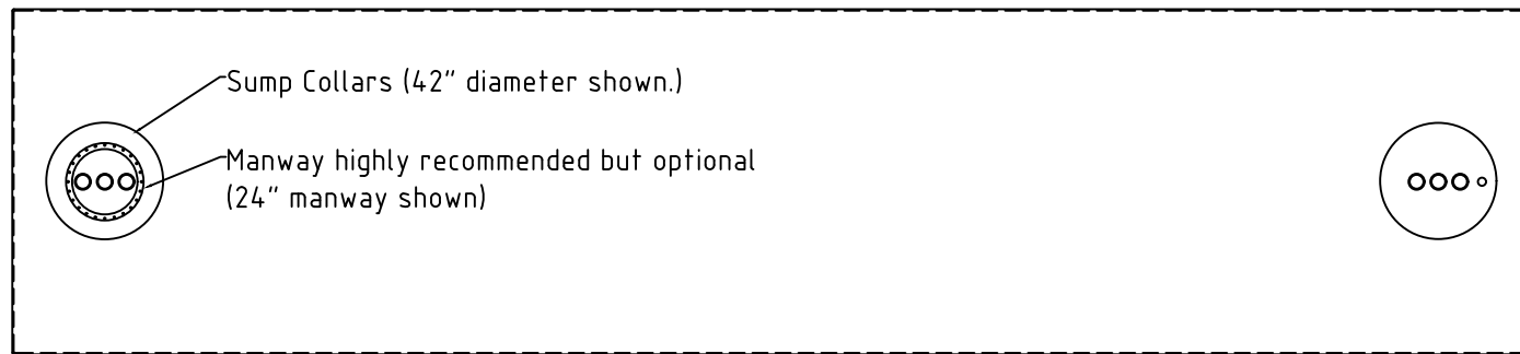
PLAN VIEW
