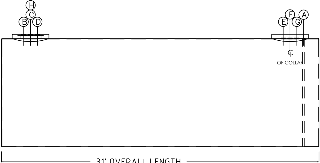
ELEVATION VIEW
