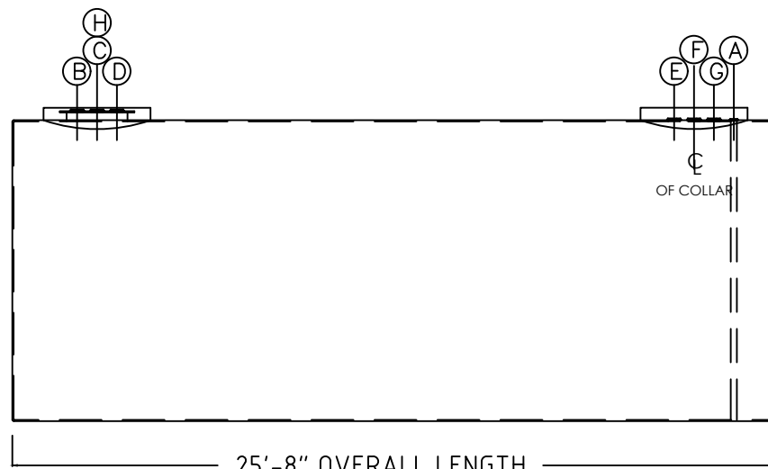
ELEVATION VIEW
