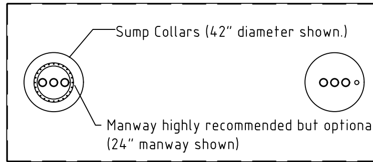
PLAN VIEW
