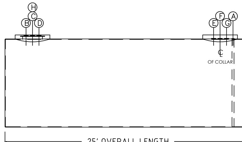
ELEVATION VIEW
