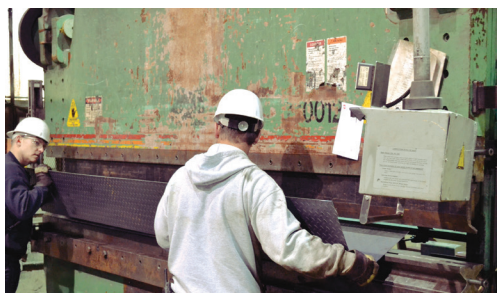
400 Ton Press Brake with 12' Bed
