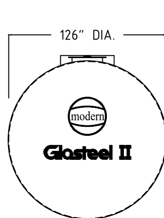
END VIEW
