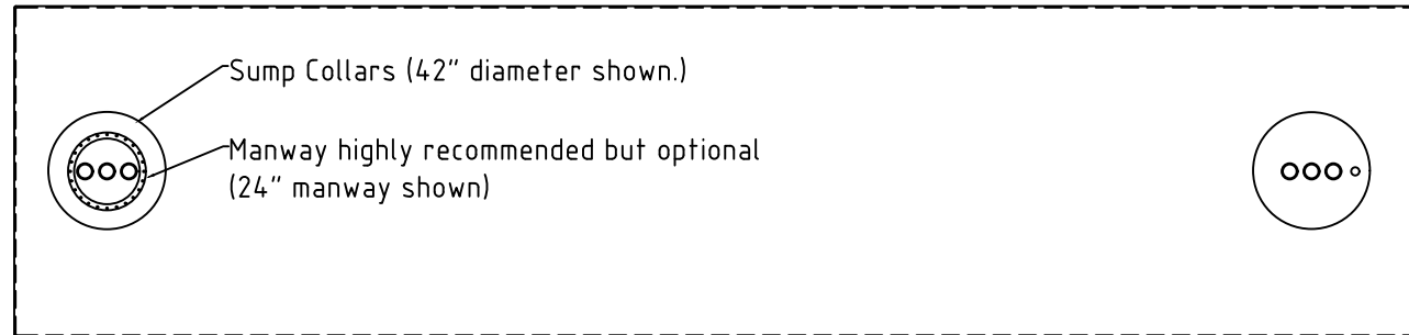
PLAN VIEW
