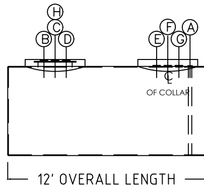
ELEVATION VIEW
