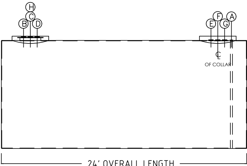
ELEVATION VIEW
