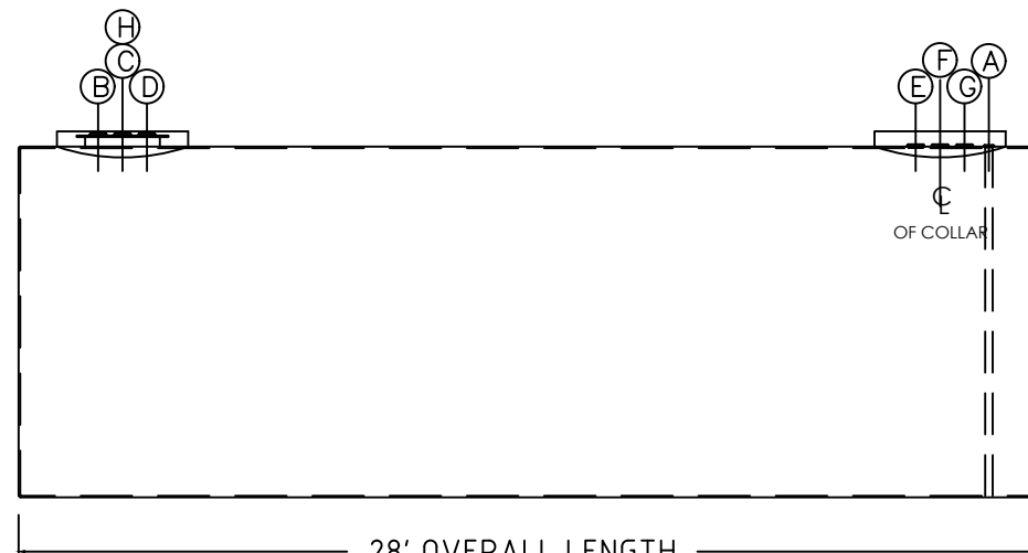
ELEVATION VIEW
